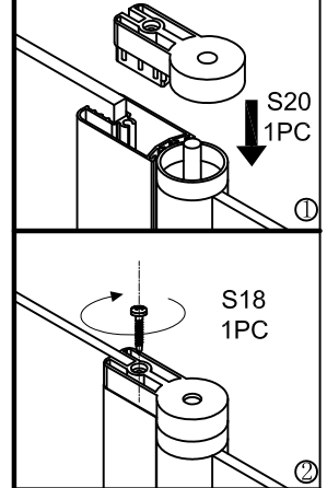
Top bracket(LH installation)
